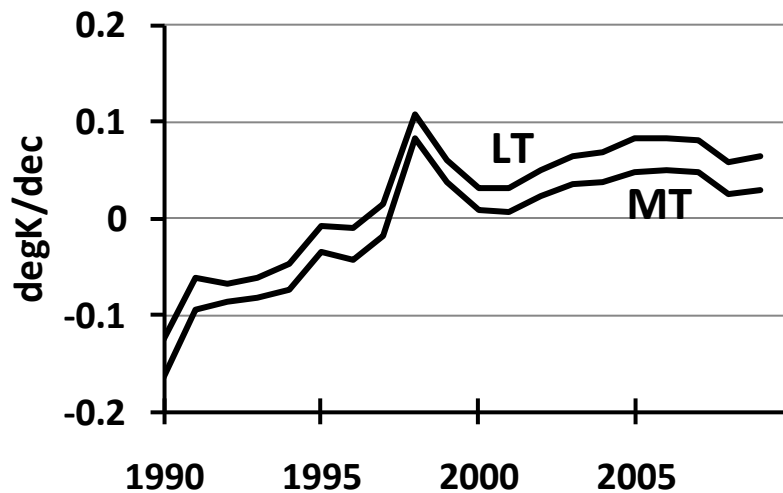
Fig. 5: Tropical Temperature trends from 1979 to Year on abscissa. RATPAC and Hadley datasets are supported by satellite results (MT minus LT); the other datasets of Fig. 4A are not – contrary to claims of Fig. 4B. Note that both LT (Lower Troposphere; main contribution from around 700 hPa) and MT (Middle Troposphere; main contribution from around 400 hPa) trends are close to zero. (Negative trends before 1997 may be a reflection of the effects of volcanic eruptions El Chichon and Pinatubo. The slightly lower MT trends may reflect the influence of stratospheric cooling.)
