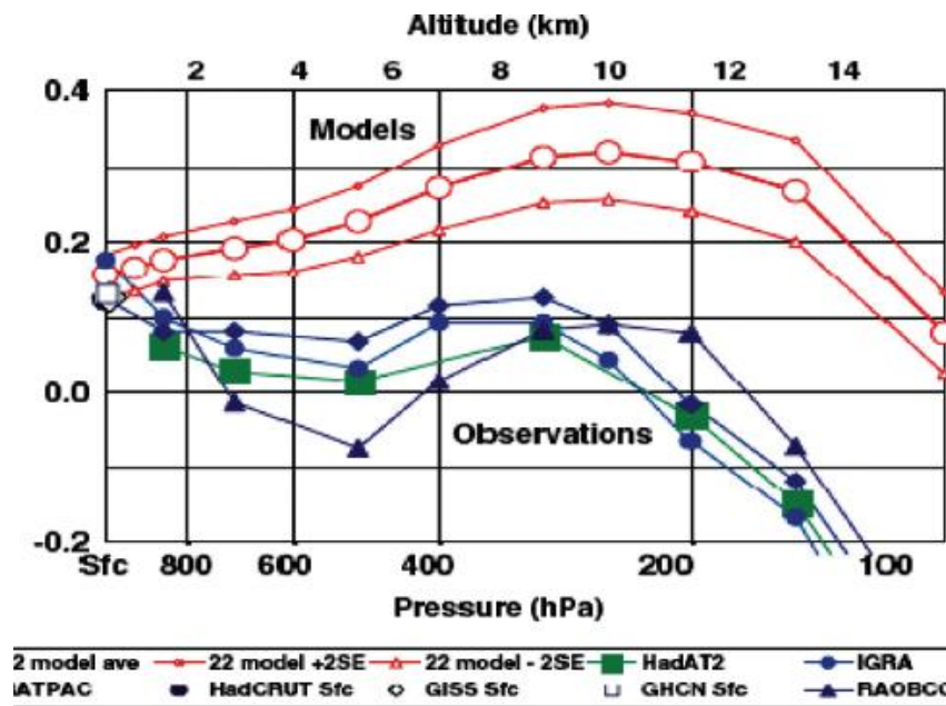
Fig. 3: Temperature trends vs altitude in the tropics [Douglass, Christy, Pearson, Singer. IJC 2007]. Note that DCPS claims a major disparity between modeled and observed (NOAA-RATPAC and Hadley) radiosonde trends.
